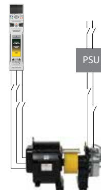
Solution using E200/E300 and Brake Control Unit
